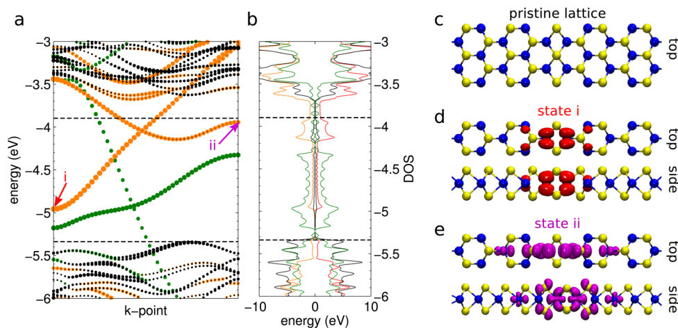
Figure 3. Atomic and electronic structures and density of states of the MTB. (a) The band structure and (b) corresponding density-of-states from a ribbon calculation with one MTB. The states are colored by the projection to different regions of the system (orange, near MTB region; green, edge region; black, bulk region). (c–e) The atomic structure of the MTB system together with the charge density isosurface visualization of wave functions of the two MTB-localized states (i) and (ii) within the gap.
