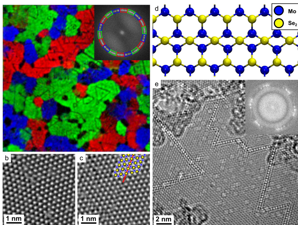
Figure 1. Atomic scale microstructure of a free-standing 2D Mo–Se layer imaged by AC-HRTEM. (a) The grain structure, with the color coding corresponding to different grain orientations. The map is generated in digital postprocessing, by selecting different orientations in the fast Fourier transform of the image and compositing the images (see Supporting Information Figure 1 for details). (b) A close-up view of a tilt grain boundary. The brighter lattice sites are Se vacancies and their concentration increases rapidly during imaging due to the electron beam. 34 (c) A close-up view of a mirror-twin-boundary (MTB) embedded within a grain, with Mo and Se positions partly overlaid with circles. (d) A structural model of the MTB. (e) An image acquired at a special focus condition placing the MoSe 2 lattice frequency at a minimum of the contrast transfer-function (see the inset FFT). At such imaging conditions, the MTBs become highly visible (the linear features), even when covered by contamination. The spots within the grains are Se vacancies.
