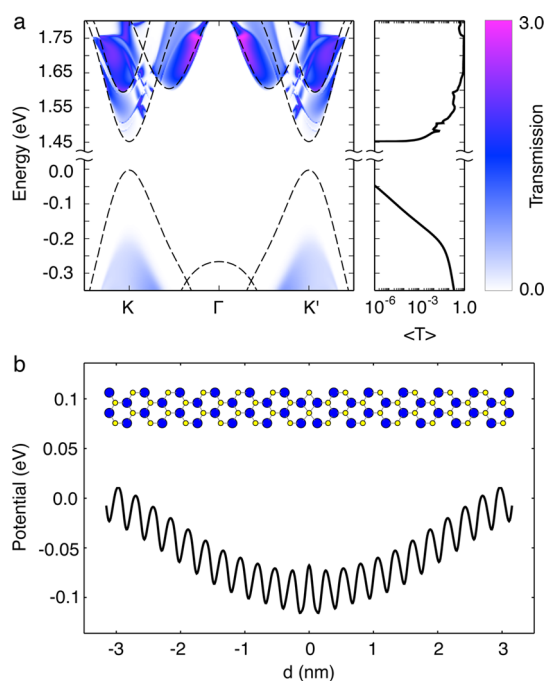
Figure 4. Electronic transport across the MTB defect. (a) Momentum and energy-resolved ballistic charge-carrier transmission probabilities across the MTB. The contours of electronic bands of pristine monolayer MoSe 2 are shown as dashed lines with the energy of the valence band maximum set as reference. Right panel presents the momentum averaged transmission \langle T \rangle on the logarithmic scale. (b) The calculated self-consistent Hartree potential along the transport direction and averaged over the planes perpendicular to it. Corresponding structure of an MTB defect is presented on the same scale.
